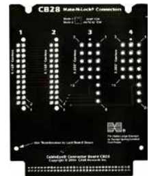
CB28 MATE-N-LOK Connectors (Item 758)
