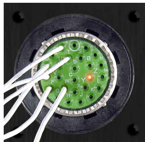
AutoBuild with Light Director Accessory Setup for 1st-Sided pinning. Target cavity is illuminated from below with LED light fiber. See "Light-Guided Assembly" on p.34.
