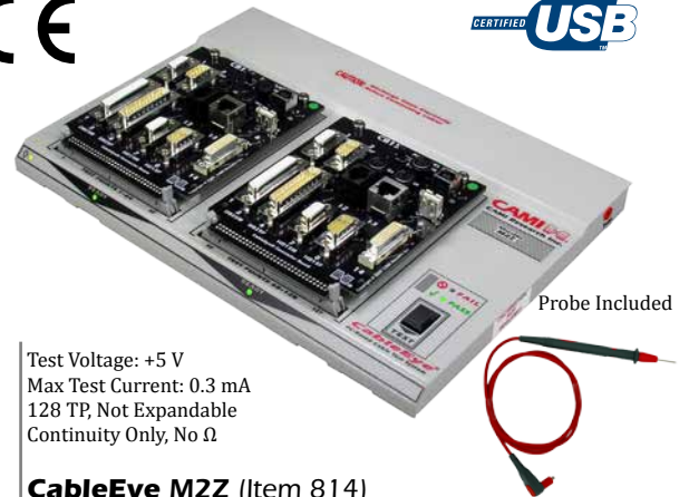
CableEye M2Z (Item 814) shown with CB15C Boards (Item 745C) Installed
