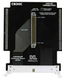
CB30C Molex 160-Pin LFH Connectors (Item 760C)
